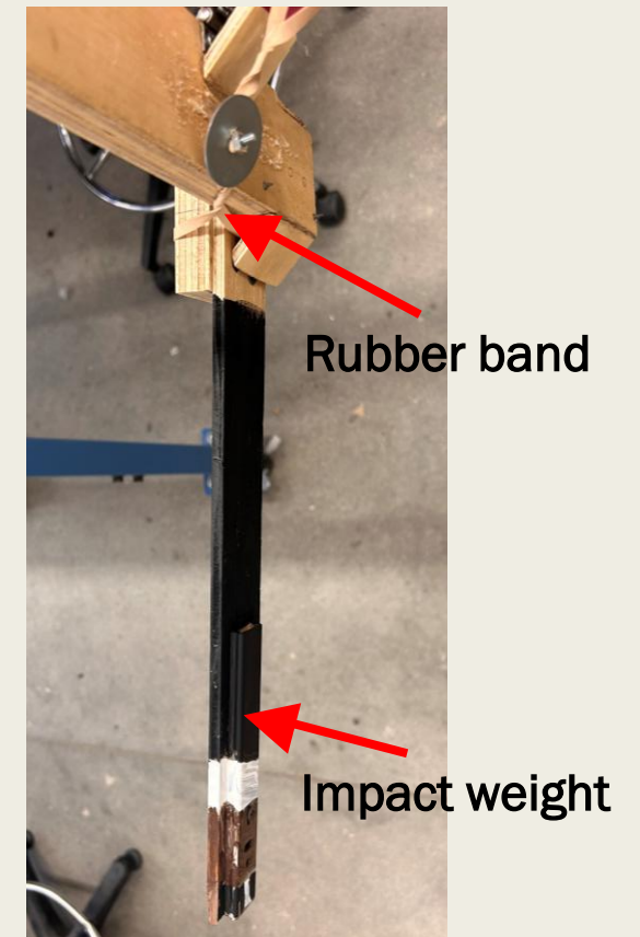
Iteration 3: Reinforced Mouse Trap Arm
