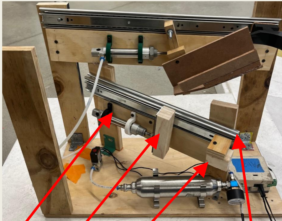
Actuator Stopper Impact Block Drawer Slider
